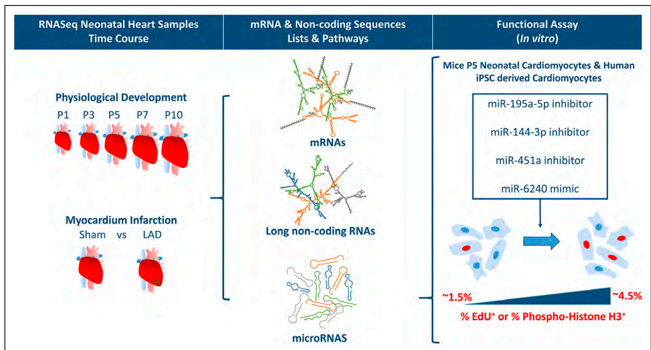
Figure. Deep molecular characterization of heart regeneration.
